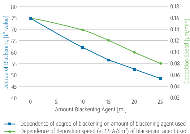
Influence of Blackening Agent
