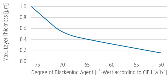
Max. Layer Thickness vs. Degree of Blackening
